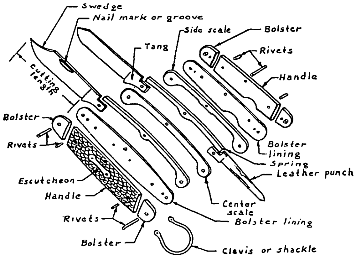
Figure 1. Knife nomenclature.
